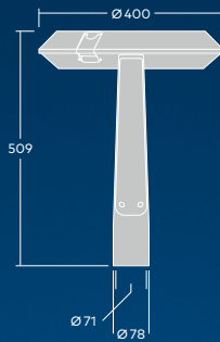
71mm diameter to fit 60mm diameter pole
