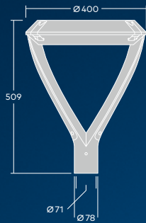
71mm diameter to fit 60mm diameter pole
