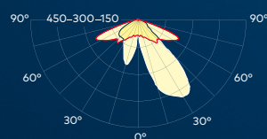
Asymmetrical Street (STR-A)
